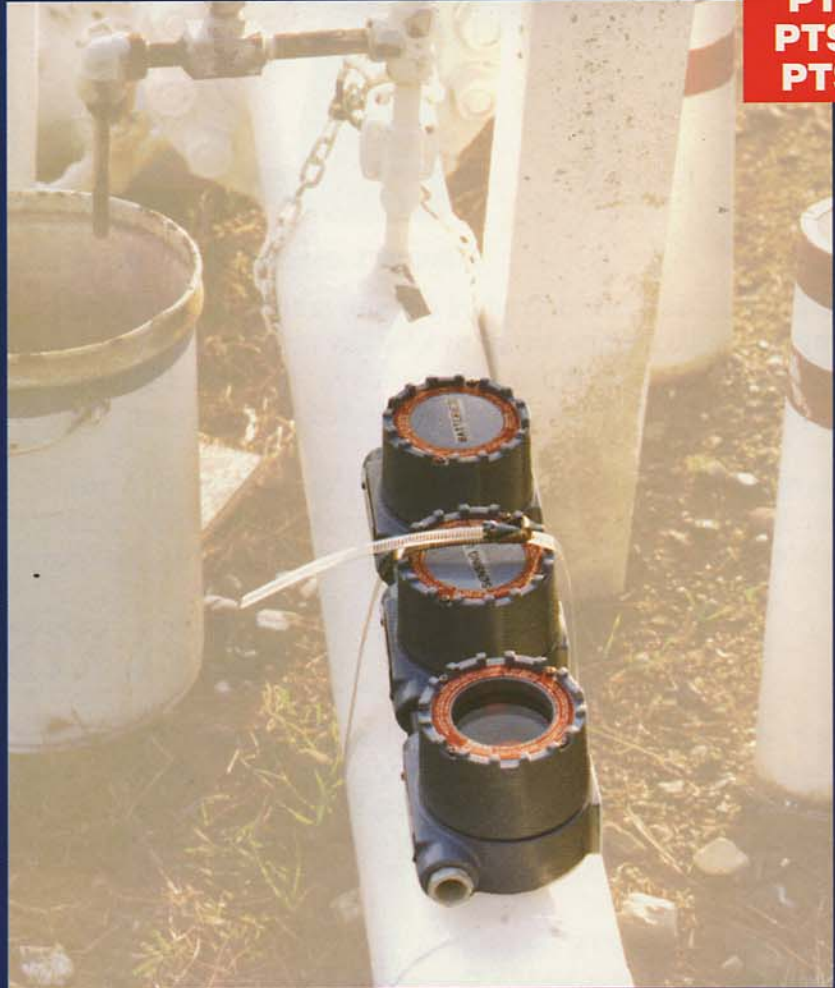
Model PTS strapped in place on pipe. In this application, the sensor signalled the launching of a series of pigs. The Model PTS was then moved to the end of the run to signal the arrival of each pig.
